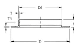
Pressed collars
