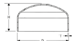
Pressed end caps
