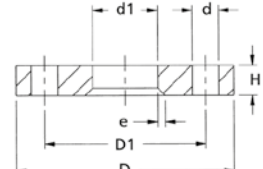
Flanges
