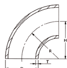
Welded 45° & 90° elbows (radius 1.5D)
