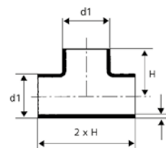
Equal tees with branch
