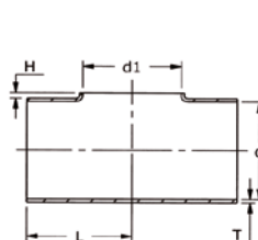
Pulled equal and reducing tees
