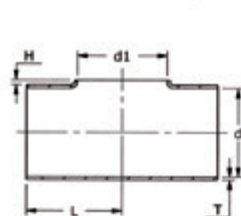
Pulled equal and reducing tees
