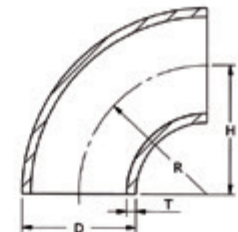
Welded 45° & 90° elbows (radius 1.5D)
